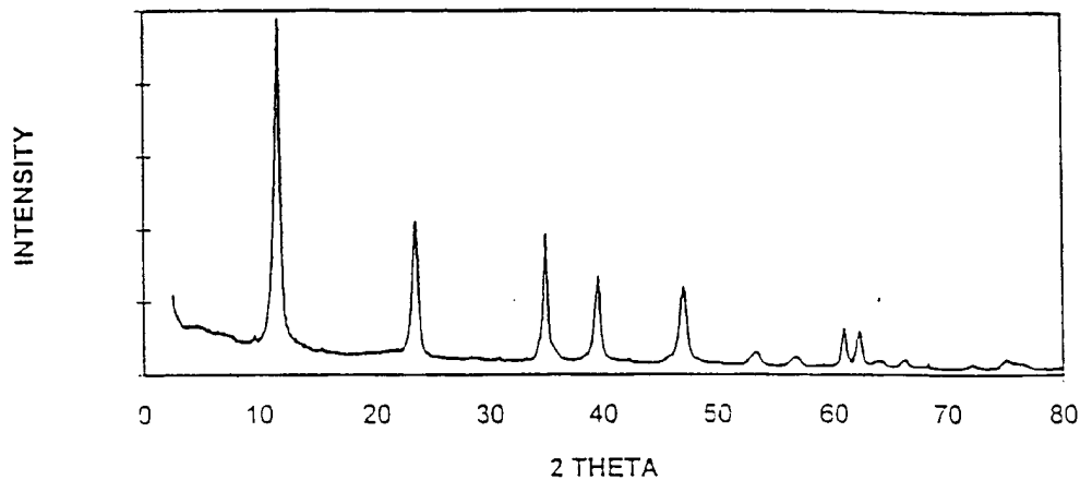
FIGURE 2: X-RAY DIFFRACTION PATTERN FOR COMMERCIAL ANIONIC CLAY
